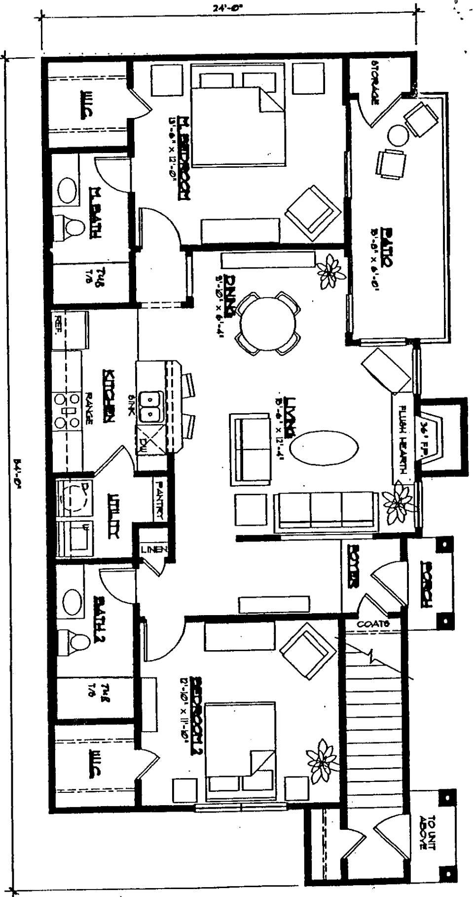
FLOOR PLAN - UNIT B2 1078 SQ.FT. SCALE : 1/8" = 1'-0"
